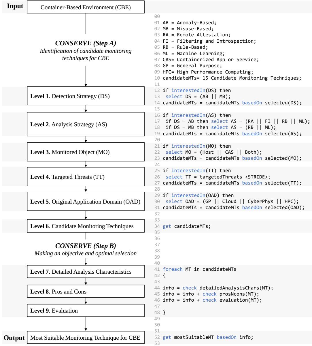
Figure 4: A flow chart ( left ) and pseudo-code ( right ) showing how to use the CONSERVE Framework
