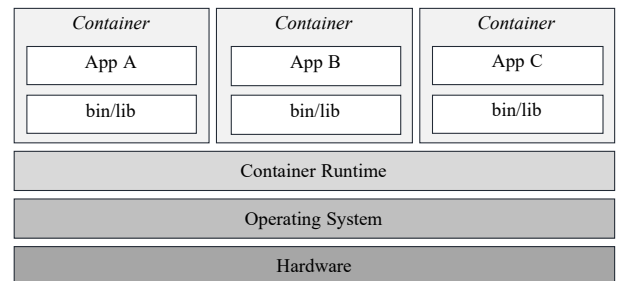
Figure 1: Architecture of container-based environments Huang and Wu (2018)
