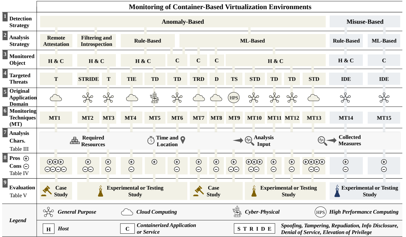
Figure 3: CONSERVE Framework for the Selection of Container Monitoring Techniques
